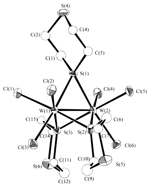
Figure 1. ORTEP representation and labeling scheme for \text{Cl}_3\text{W}(\mu\text{-1,4-dithiane})_3\text{WCl}_3 ( 1 ). Hydrogen atoms omitted for clarity.
