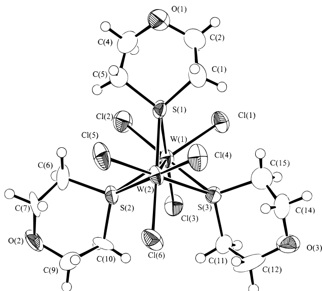
Figure 2. ORTEP representation and labeling scheme for \text{Cl}_3\text{W}(\mu\text{-1,4-thioxane})_3\text{WCl}_3 ( 2 ).
