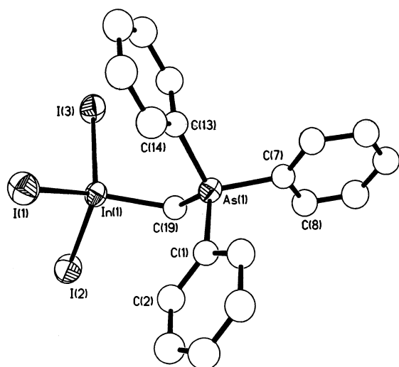
Fig. 2. Molecular structure of \text{I}_3\text{InCH}_2\text{As}(\text{C}_6\text{H}_5)_3 , 4 , (ORTEP diagram), with atoms shown as 30% probability ellipsoids. Hydrogen atoms have been omitted for clarity.
