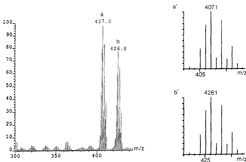
Fig. 2. FAB mass spectrum in the high molecular weight region of 5 with expansions of the two most intense groupings at m/e = 407 , [\text{Pd}(\text{1})]^{2+} and m/e = 426 , [\text{PdF}(\text{1})]^+ . The latter arises from the extraction of \text{F}^- from \text{BF}_4^- .
