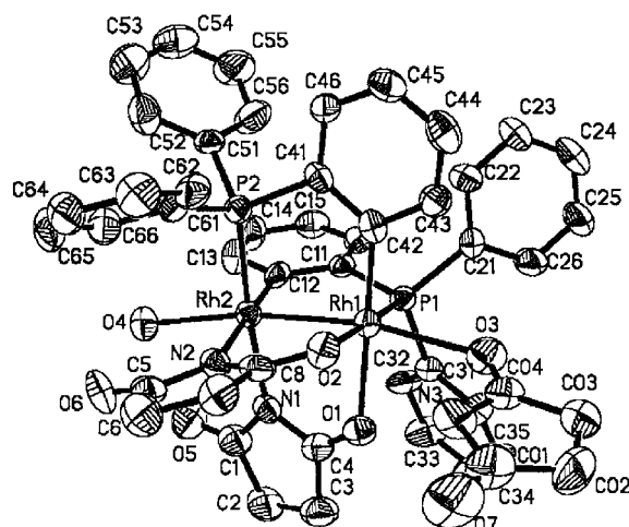
Figure 1. Molecular view of \text{Rh}_2(\text{C}_4\text{H}_4\text{NO}_2)_2[(\text{C}_6\text{H}_4)\text{P}(\text{C}_6\text{H}_5)_2]_2 \cdot (\text{H}_2\text{O})(\text{C}_4\text{H}_5\text{NO}_2) ( 3 ), with the H atoms omitted for clarity. Selected bond distances (Å) and angles (deg) are Rh1–Rh2 2.5551(7), Rh1–C42 1.970(7), Rh1–P1 2.2052(16), Rh2–C12 1.997(6), Rh2–N1 2.119(5), C42–Rh1–O1 172.50(19), O2–Rh1–O3 90.00(16), and C12–Rh2–O4 90.9(2).
