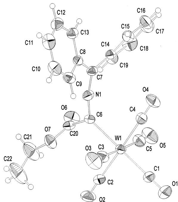
Fig. 1. ORTEP projection of the tungsten complex 6c with the atom numbering scheme.
