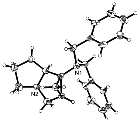
Figure 1. Molecular structure of compound (1 aS ,6 aS ,6 bR )- 16 in the crystal. [22]
