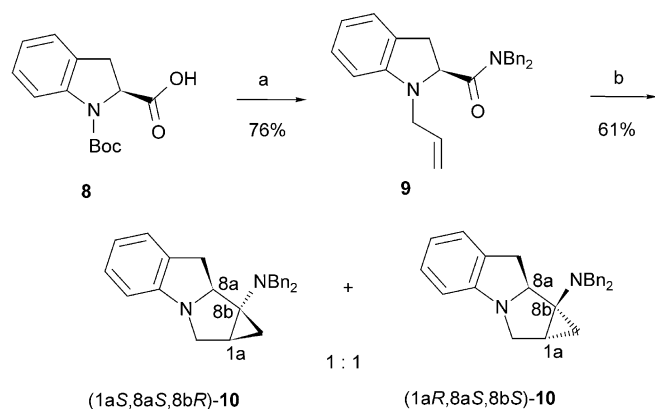
Scheme 3. a) 1) \text{HNBn}_2 , DCC, HOBT, \text{CH}_2\text{Cl}_2 , 20°C, 2 d; 2) TFA, \text{CH}_2\text{Cl}_2 , 20°C, 12 h; 3) allyl bromide, \text{K}_2\text{CO}_3 , MeCN, 60°C, 16 h; b) cHexMgBr, [\text{MeTi}(\text{OiPr})_3] , THF, 20°C, 12 h.
