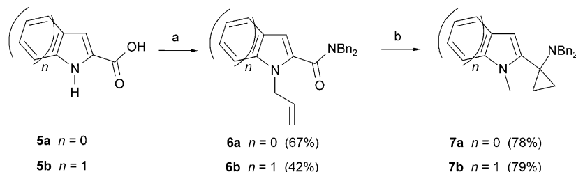
Scheme 2. a) 1) \text{HNBn}_2 , DCC, HOBT, \text{CH}_2\text{Cl}_2 , 20°C, 2 d; 2) allyl bromide, \text{K}_2\text{CO}_3 , MeCN, 60°C, 16 h. b) cHexMgBr, [\text{MeTi}(\text{OiPr})_3] , THF, 20°C, 12 h.
