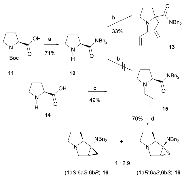
Scheme 4. a) 1) \text{HNBn}_2 , DCC, HOBT, \text{CH}_2\text{Cl}_2 , 20°C, 2 d; 2) TFA, \text{CH}_2\text{Cl}_2 , 20°C, 12 h; b) Allyl bromide, \text{K}_2\text{CO}_3 , MeCN, 60°C, 16 h; c) 1) Allyl bromide, KOH, i\text{PrOH} , 40°C, 22 h; 2) \text{HNBn}_2 , DCC, HOBT, \text{CH}_2\text{Cl}_2 , 20°C, 1 d; d) cHexMgBr, [\text{MeTi}(\text{OiPr})_3] , THF, 20°C, 12 h.
