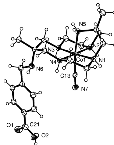
Fig. 1 View of [\text{Co}(\text{HL}^{10})(\text{CN})]^{2+} (30% ellipsoids). Selected bond lengths (Å) Co(1)–C(13) 1.893(3), Co(1)–N(1) 1.957(3), Co(1)–N(2) 1.947(3), Co(1)–N(3) 1.958(2), Co(1)–N(4) 1.958(3), Co(1)–N(5) 1.979(3), C(21)–O(1) 1.203(5), C(21)–O(2) 1.327(5).
