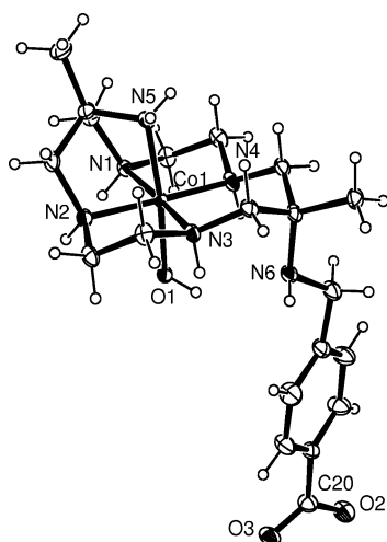
Fig. 2 View of [\text{CoL}^{10}(\text{OH})]^+ (30% ellipsoids). Selected bond lengths (Å) Co(1)–O(1) 1.910(3), Co(1)–N(1) 1.949(4), Co(1)–N(2) 1.950(4), Co(1)–N(3) 1.943(4), Co(1)–N(4) 1.954(4), Co(1)–N(5) 1.967(4), C(20)–O(2) 1.265(7), C(20)–O(3) 1.257(7).
