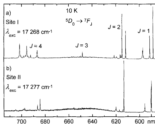
Figure 6. Part of the laser-excited emission spectrum of [\text{Eu}(\text{L}^5)_2(\text{TfO})_2(\text{OH}_2)]\text{TfO} ( 1 ) at 10 K upon selective excitation at a) \lambda_{\text{exc}} = 17\,268\text{ cm}^{-1} (site I) and b) \lambda_{\text{exc}} = 17\,277\text{ cm}^{-1} (site II).
