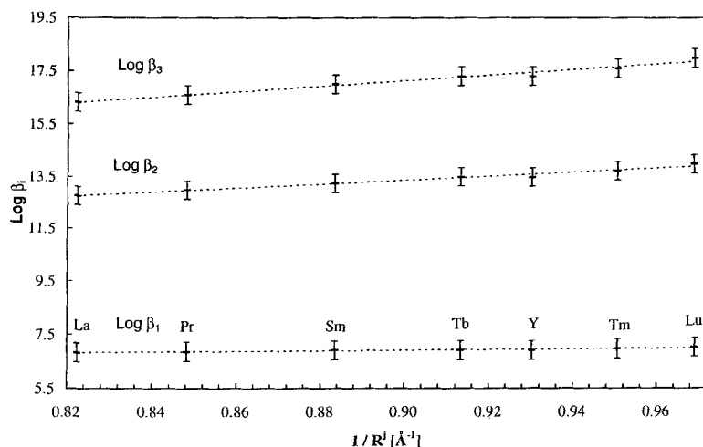
Figure 1. Stability constants log( \beta_1^{Ln} ) for [Ln( L 5 ) 3 ] 3+ ( i = 1–3) vs. 1/ R i ( R i ionic radii of nonacoordinate Ln III ) [19].
