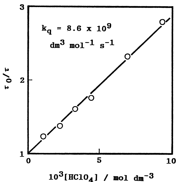
Fig. 1. Plot of \tau_0/\tau vs. [\text{HClO}_4] for the quenching of ^1\text{AcrHR}^* ( \text{R} = 1\text{-naphthylmethyl} ) by \text{HClO}_4 in deaerated MeCN containing \text{H}_2\text{O} ( 0.50 \text{ mol dm}^{-3} ) at 298 K.
