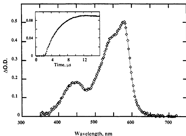
Figure 3. Transient absorption spectrum measured 1 \mu s after 308-nm excitation of benzocyclobutenedione in toluene containing 0.05 M pyridine. Inset: Growth of the transient absorption at 550 nm for a similar sample containing 0.133 mM pyridine.
