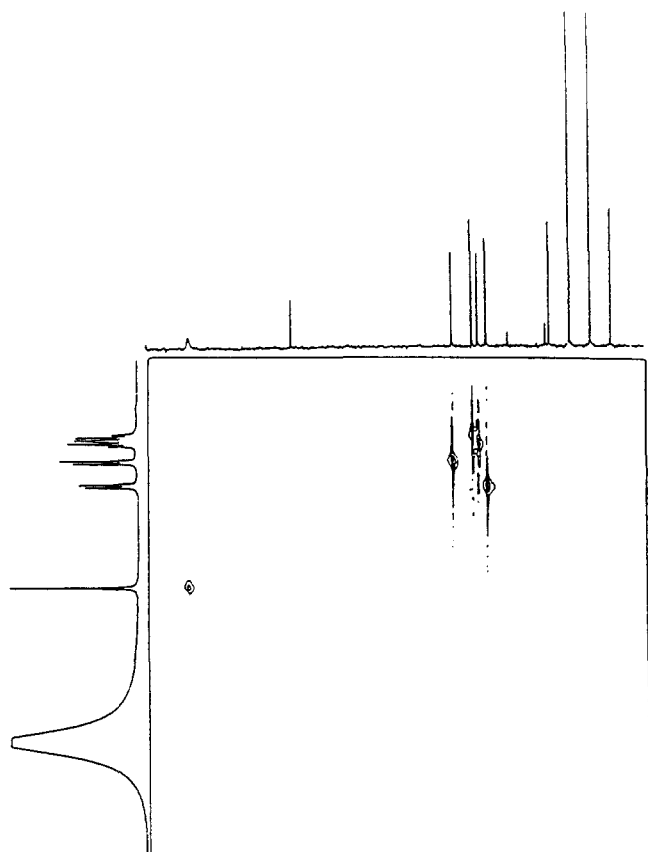
Figure 7. ^{13}\text{C} NMR spectrum of carbocation VIII in dichloromethane- d_2 .
