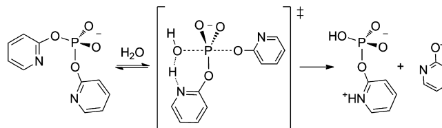
Scheme 9. Mechanism iv: S N 2(P) Mechanism for Hydrolysis Using a Single Water Molecule with General Base Catalysis by a Nitrogen Atom of the Non-Leaving Group
