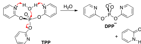
Scheme 2. Suggested Special Mechanism for “Efficient” Intramolecular GBC of the Hydrolysis of TPP 1
