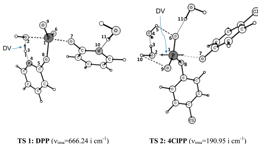
Figure 5. Optimized structures for the transition states TS for the hydrolysis reactions of DPP and 4ClPP. For a key to the atom numbering, see Scheme 10. The roles of the water molecules are discussed in detail in the following section.
