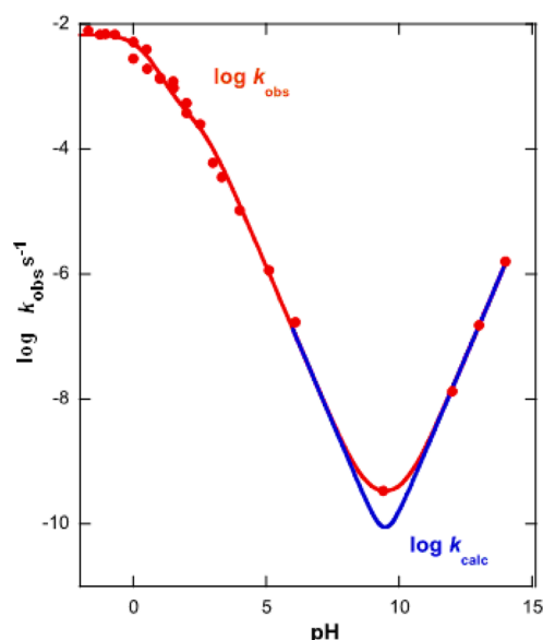
Figure 1. pH–(log) rate profile for the hydrolysis of DPP at 25 °C and ionic strength 1.0 M (KCl). The points for k_{\text{obs}} are experimental; the curves are calculated using the rate constants and \text{pK}_a 's shown in Table 1 but setting k_0 to zero for k_{\text{calc}} . For full data see the Supporting Information.
