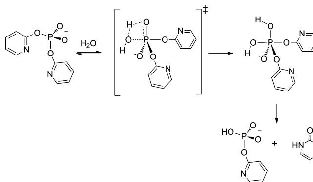
Scheme 9. Mechanism iv: S N 2(P) Mechanism for Hydrolysis Using a Single Water Molecule with General Base Catalysis by a Nitrogen Atom of the Non-Leaving Group
