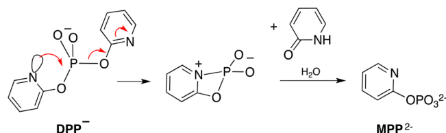
Scheme 6. Mechanism (ii): Intramolecular Nucleophilic Catalysis of the Hydrolysis of DPP by Pyridine Nitrogen a
