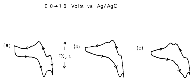
Figure 8. Cyclic voltammograms at a mercury electrode in acetone at scan rates of 50 \text{ V s}^{-1} and at 20^\circ \text{C} for (a) \text{Fe}(\text{CO})_4\text{PPh}_3 , (b) \text{Fe}(\text{CO})_4\text{AsPh}_3 , and (c) \text{Fe}(\text{CO})_4\text{SbPh}_3 (concentration approximately 10^{-3} \text{ M} ).
