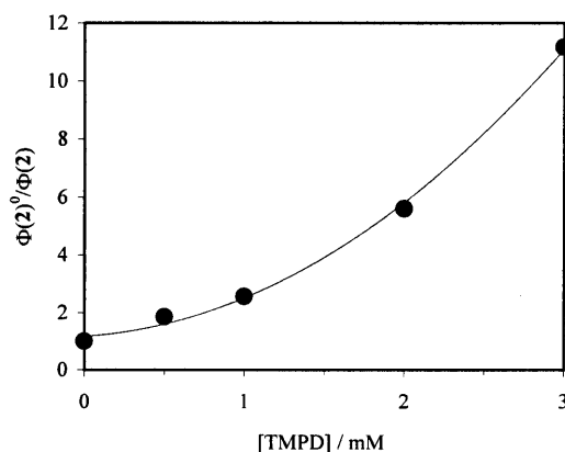
Figure 1. Dependence of the yield of 2 upon the TMPD concentration in the photolysis of 1 in MeCN–MeOH (9:1)
