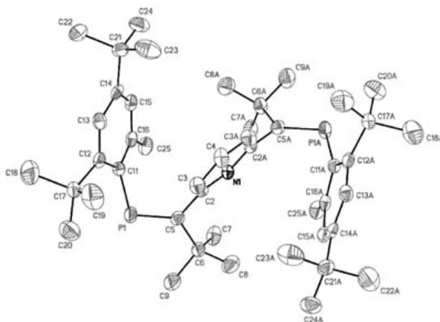
FIGURE 2 ORTEP drawing of 2,6-bis[1-(2',4'-di- tert -butyl-6'-methylphenyl)phosphinidene-2'',2''-dimethylpropyl]-pyridine ( 7 ).
