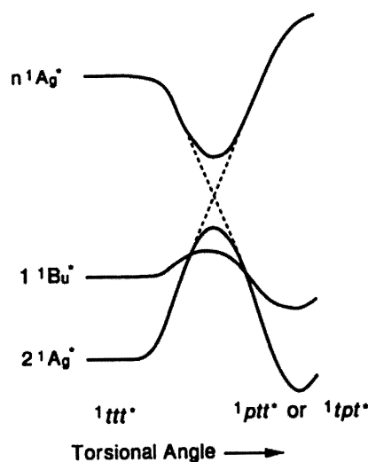
Figure 4. Possible torsional relaxation pathways leading to 1^1ttt -DPH* photoisomerization (schematic, not to scale).
