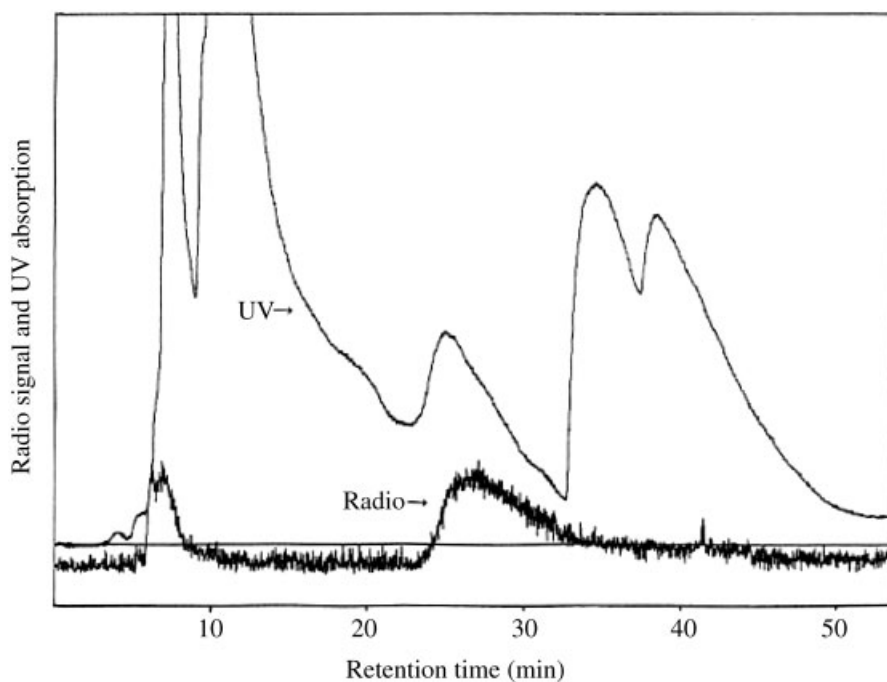
Figure 3. Semi-preparative HPLC separation of [ 18 F]BF-108
