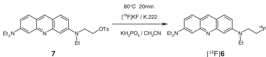
Figure 2. Synthesis of [ 18 F]BF-108
