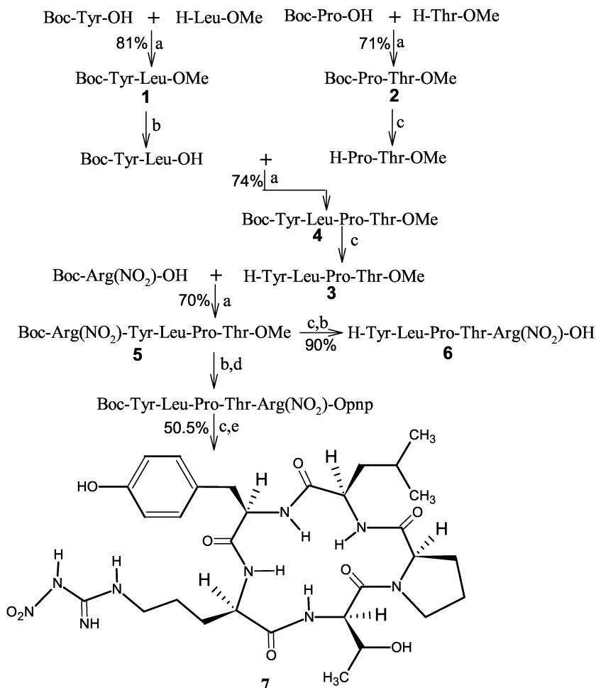
Scheme 1. a = DCC, NMM, HOBT, DCM, RT/36 h; b = LiOH, THF:H 2 O(1:1), RT/1 h; c = TFA, CHCl 3 , RT/1 h; d = p -nitrophenol (pnp), DCC, CHCl 3 , RT/12 h; e = pyridine, CHCl 3 , 10 days/0 °C.
