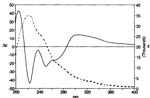
Fig. 2. Absorption (-----) and CD (——) spectrum of [\text{Rh}(\text{COD})((R)\text{-BNDA})]\text{BF}_4 in methanol.
