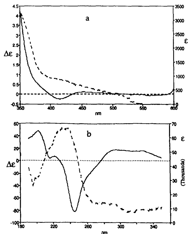
Fig. 3. Absorption (-----) and CD (——) spectrum of [\text{Ir}(\text{COD})((R)\text{-BNDA})]\text{BF}_4 in methanol: (a) between 600 and 350 nm; (b) between 360 and 190 nm.
