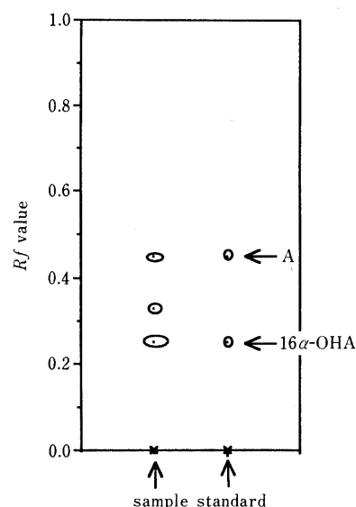
Fig. 1. Thin-Layer Chromatogram of Products Obtained by Incubation of Non-labeled A with a Strain of Streptomyces roseochromogenes
