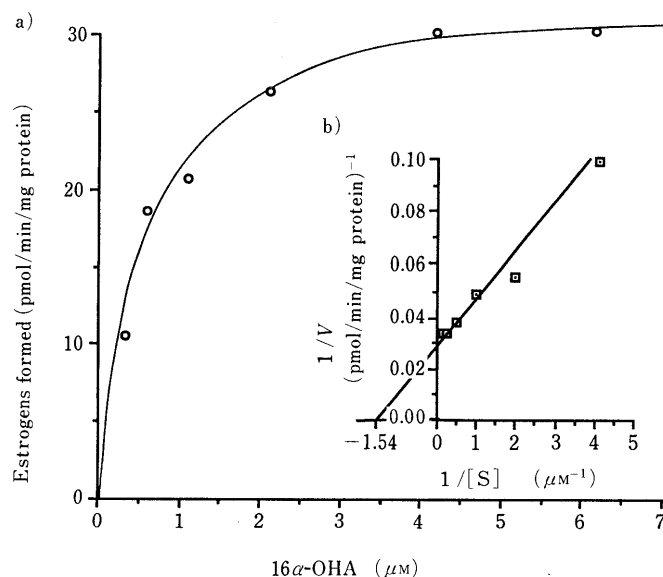
Fig. 4. Lineweaver-Burk Plot of Aromatization of [1\beta\text{-}^3\text{H}] 16\alpha\text{-OHA}
