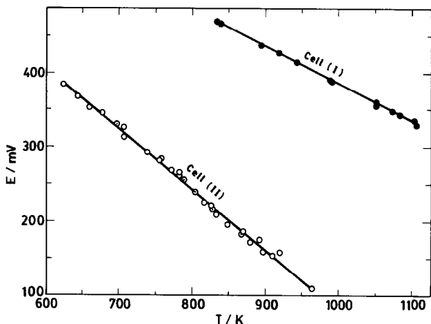
Fig. 1. Experimental e.m.f. results for cells (I) and (II) (●) cell (I): Pt,C,Te(I),NiTeO 3 ,NiO test electrode; (○) cell (II): Pt,C,NiTeO 3 ,Ni 3 TeO 6 ,NiO test electrode.
