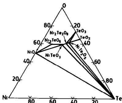
Fig. 2 Phase equilibrium diagram of Ni-Te-O system at 850 K
