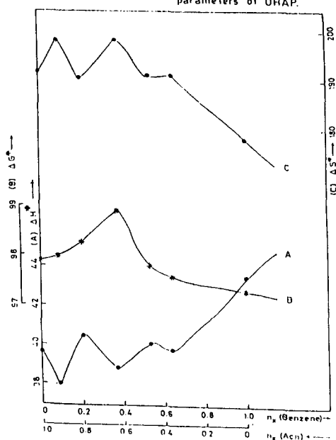
Fig. v Solvent effects on activation parameters of OHAP.
