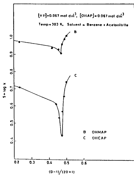
Fig. III Kirkwoods' Plots
