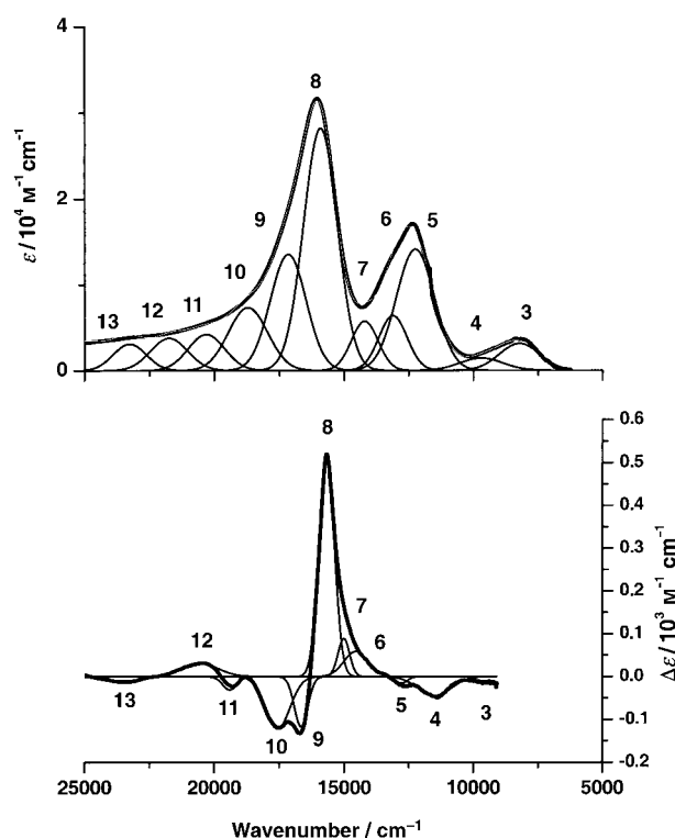
Figure 16. Deconvoluted electronic absorption spectrum [\text{Co}(\text{L}_\text{N})_2]^0 (top) and its magnetic circular dichroism (MCD) spectrum (bottom) recorded at 1.8 K and 5.0 T.
