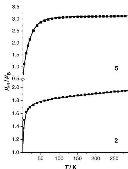
Figure 3. Temperature dependence of the magnetic moment of solid 5 (top) and 2 (bottom). The solid lines represent best fits with parameters for 5 : S = 1 ; |D| = 57 \text{ cm}^{-1} ; g = 2.25 , and for 2 : S = 1/2 , g_{\text{iso}} = 2.09 , \chi_{\text{TIP}} = 250 \times 10^{-6} \text{ emu} ; \theta = -3.0 \text{ K} .
