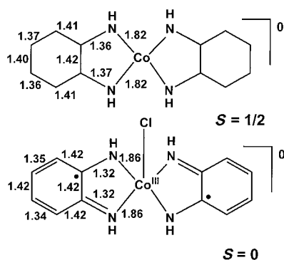
Figure 1. Schematic structures with bond lengths in Å of square-planar [\text{Co}(\text{L}_\text{N})_2]^0 from reference [3] (top) and square-base pyramidal [\text{Co}^{\text{III}}(\text{L}_\text{N})_2\text{Cl}] from reference [3] (bottom). The experimental errors from the room-temperature crystal structures are \sim \pm 0.03 Å ( \equiv 3\sigma ) for the former and \pm 0.015 Å for the latter.
