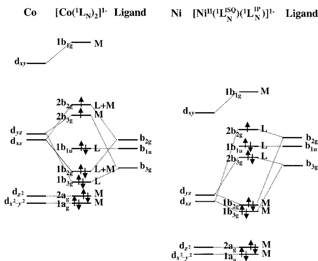
Figure 15. MO schemes of [\text{Co}(\text{L}_\text{N})_2]^{1-} and of [\text{Ni}^{\text{II}}(\text{L}_\text{N}^{\text{ISO}})(\text{L}_\text{N}^{\text{IPI}})]^{1-} .
