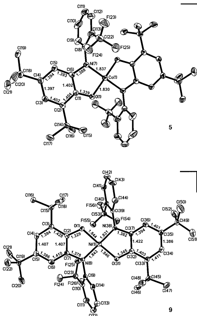
Figure 7. Structures of the monoanions [\text{Co}^{\text{III}}(^4\text{L})_2]^- in crystals of 5 (top) and [\text{Ni}^{\text{II}}(^4\text{L})(^4\text{L})^-] in crystals of 9 (bottom). The error of the C–N, C–O, and C–C bond lengths is \pm 0.01 \text{ \AA} ( 3\sigma ) for 5 and \pm 0.015 \text{ \AA} for 9 .
