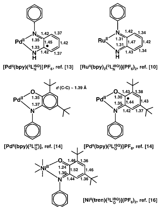
Figure 4. Average C–O, C–N, and C–C distances in \text{\AA} in complexes containing (\text{}^2\text{L}_\text{N})^{n-} or (\text{}^3\text{L}_\text{O})^{n-} ligands ( n=2, -1, -0 ).
