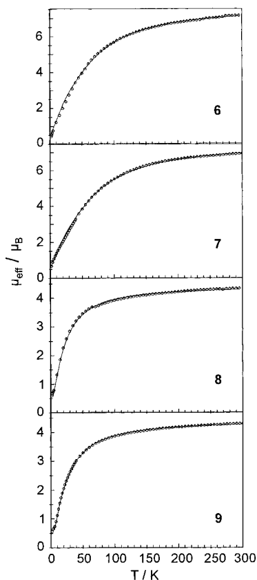
Figure 3. Temperature dependence of the magnetic moment, \mu_{\text{eff}} , per dinuclear unit of powdered samples of complexes 6–9. The solid lines represent best fits obtained as described in Figure 2.
