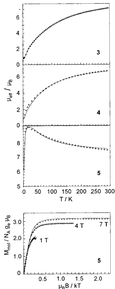
Figure 2. Temperature dependence of the magnetic moment, \mu_{\text{eff}} , per dinuclear unit of powdered samples of complexes 3–5 measured at 1 T. Bottom: Magnetization data of 5 measured at various fields. The solid lines represent best fits to the spin-Hamiltonian eq 1 with parameters listed in Table 6.
