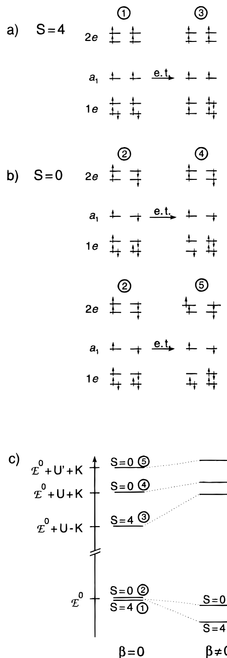
Figure 8. Generation of possible excited states 3–5 by one-electron transfer steps in the 1e orbitals assuming (a) parallel 1 or (b) antiparallel 2 spin alignment in the ground state of tris( \mu -chloro)diferrous complexes. (c) Relative energies of the ground and excited states without interaction between the metal ions ( \beta = 0 ) and with such interaction ( \beta \neq 0 ).
