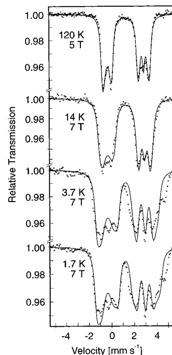
Figure 6. Magnetic Mössbauer spectra of solid [(thf) 6 Fe 12 (μ-Cl) 3 ][SnCl 5 (thf)]. The solid lines represent spin-Hamiltonian simulations with S i = 2, η = 0; J = -0.8 cm -1 , D i = +3.5 cm -1 , g = 2.0; A i / g N μ N = (-1.0, -10.2, -19.7) T; ΔE Q = -3.27 mm s -1 (-3.19 mm s -1 at 120 K), and δ = 1.3 mm s -1 (1.27 mm s -1 at 120 K).
