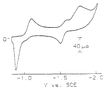
Figure 2. Cyclic voltammogram of [\text{Ir}(\text{phen})(\text{cod})]\text{ClO}_4 in 0.1 M TEAP in acetonitrile; scan rate 200 mV/s.
