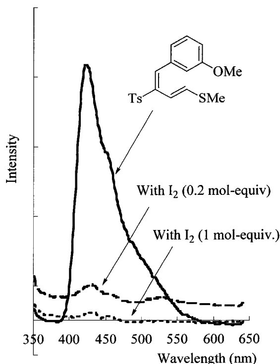
FIGURE 2 PL spectrum of 1e (10 -2 M in CH 3 CN) in the absence and presence of I 2 (excitation at 332 nm).
