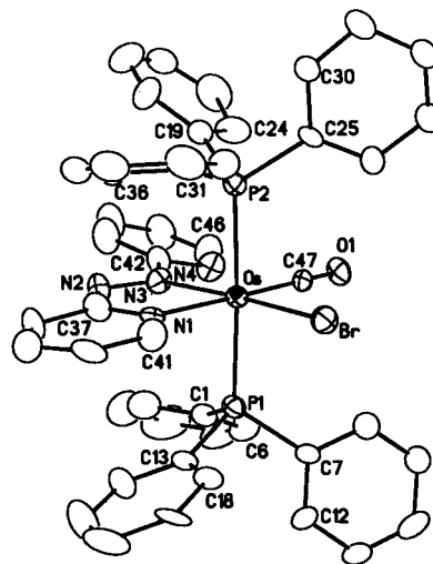
Figure 1. Molecular structure of [\text{Os(abp}^{\prime-})\text{(Br)(CO)(PPh}_3)_2] ( 6b ) showing 30% probability ellipsoids.
