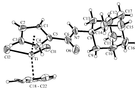
Figure 2. Projection of the molecular geometry of 8b (with unsystematical atom numbering scheme). Selected bond lengths (Å) and angles (deg): Ti–Cl1, 2.356(3); Ti–Cl2, 2.345(3); Ti–C1, 2.429(9); Ti–C2, 2.418(10); Ti–C3, 2.348(10); Ti–C4, 2.364(9); Ti–C5, 2.380(9); Ti–C18, 2.343(13); Ti–C19, 2.382(12); Ti–C20, 2.350(11); Ti–C21, 2.351(11); Ti–C22, 2.325(12); C5–C6, 1.481(14); C6–O6, 1.235(12); C6–N7, 1.348(13); N7–C8, 1.472(13); O6–C6–N7, 124.7(10); O6–C6–C5, 119.6(10); N7–C6–C5, 115.7(9); C6–N7–C8, 126.0(9); Cl2–Ti–Cl1, 95.69(11).
