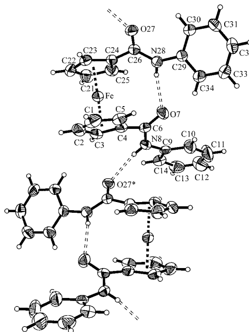
Figure 1. View of the molecular structure and association pattern of 6d in the solid state (with unsystematical atom numbering scheme). Selected bond lengths (Å) and angles (deg): Fe–C1, 2.046(6); Fe–C2, 2.047(6); Fe–C3, 2.036(6); Fe–C4, 2.029(5); Fe–C5, 2.025(6); Fe–C21, 2.040(6); Fe–C22, 2.046(6); Fe–C23, 2.039(5); Fe–C24, 2.036(5); Fe–C25, 2.024(6); C4–C6, 1.481(8); C6–O7, 1.236(6); C6–N8, 1.339(7); N8–C9, 1.420(7); C24–C26, 1.477(7); C26–O27, 1.223(6); C26–N28, 1.346(7); N28–C29, 1.422(7); O7–C6–N8, 123.4(5); O7–C6–C4, 121.8(5); N8–C6–C4, 114.8(5); C6–N8–C9, 127.6(5); O27–C26–N28, 124.1(5); O27–C26–C24, 120.3(5); N28–C26–C24, 115.7(5); C26–N28–C29, 126.3(5).
