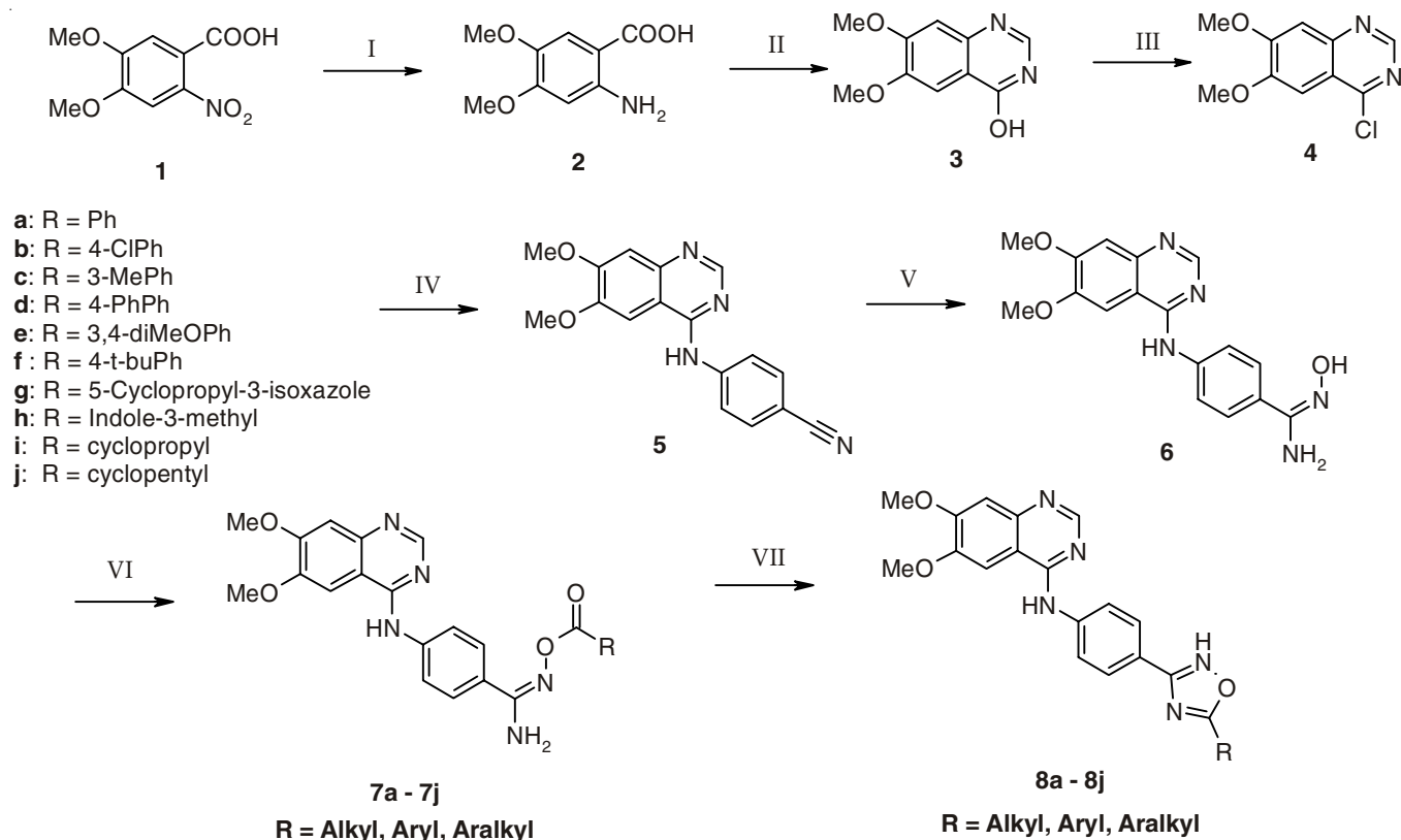
Scheme-I: Conditions and reagents: (I) 10 % Pd/C, H 2 gas, MeOH, 25 °C, 5 h; (II) Formamidine acetate, 2-methoxyethanol, 120 °C, 12 h; (III) POCl 3 , 100 °C, 2 h; (IV) 4-cyanoaniline, 2-propanol, 80 °C, 4 h; (V) NH 2 OH·HCl, KOH, EtOH, 80 °C, 12 h; (VI) R-COOH, EDC·HCl, HOBt, DMPA, 25 °C, 1 h; (VII) DBU, DMF, 80 °C, 12 h
