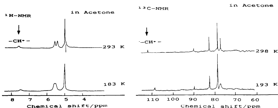
Fig. 5. ^1\text{H} NMR spectra and ^{13}\text{C} NMR spectra of 5 at indicated temperatures.
