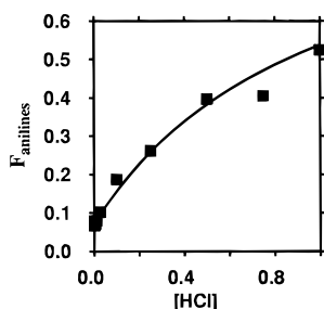
Figure 4. Yield of aniline products {%(23 + 24 + 25):100} as a function of HCl concentration. The points are experimental. The line has been drawn according to eq 9 using the parameters given in the text.
