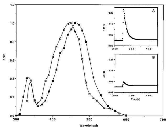
Figure 2. Absorption spectra following 248 nm irradiation of 2 \times 10^{-5} M solutions of 4-biphenyl azide (■) and 2-fluorenyl azide (□) in 1:4 (v/v) acetonitrile–water. Optical density units in the main figure have been normalized so that the maximum \Delta OD is 1. The inserts show the kinetic traces at 460 nm for 4-biphenyl azide in 1:4 acetonitrile–water (A) and 4:1 acetonitrile–water (B).
