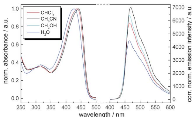
Fig. 1 UV-vis absorption and fluorescence emission spectra of polymer 5 in various solvents (25 °C). Absorption spectra are scaled to the same optical density, while emission spectra are corrected and normalized.
