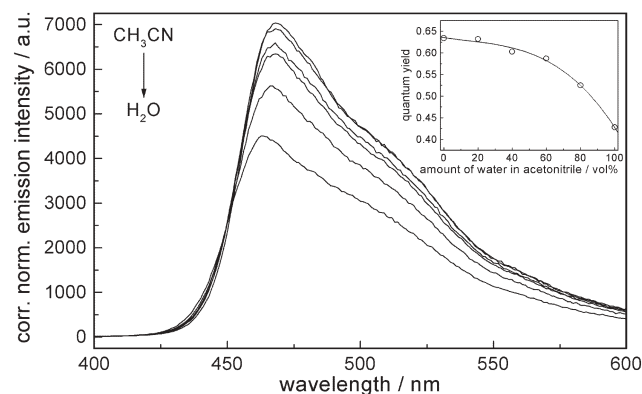
Fig. 2 Fluorescence emission spectra of polymer 5 in acetonitrile–water solvent mixtures (25 °C). The inset shows the calculated quantum yields as a function of solvent composition (the line obtained from the non-linear least squares fit of the data is included as a guide to the eye).
