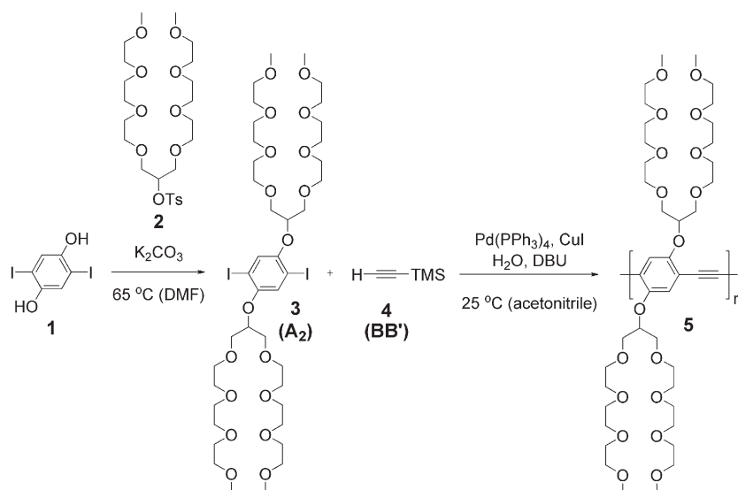
Scheme 1 Synthesis of water-soluble PpPE derivative 5 from readily available monomers 3 and 4 via an A 2 + BB' polycondensation route.
