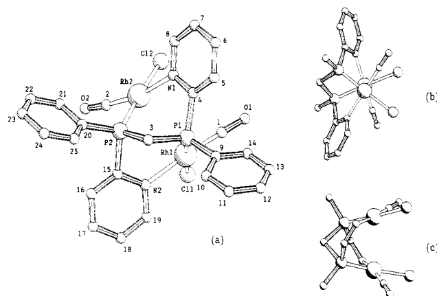
Figure 1. PLUTO drawings of \text{DPyPM}[\text{Rh}(\text{CO})\text{Cl}]_2 . All hydrogen atoms have been omitted; in parts b and c, some phenyl and pyridyl carbons have been omitted as well.
