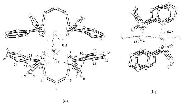
Figure 2. PLUTO drawing of the (\text{meso-DPyPP})_2\text{Rh}_2\text{Cl}_2^{2+} dication. Hydrogen atoms are not shown; in part b, most phenyl carbons have been omitted for clarity as well.
