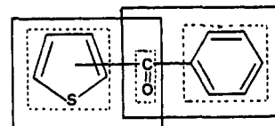
Figure 10. The total absorption of the benzoylthiophenes can be divided into transitions within five more or less independent chromophores.
