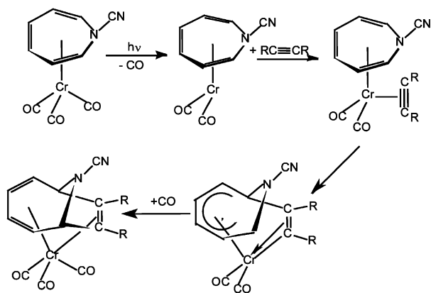
Scheme 1. The proposed mechanism for the formation of complexes 3a and 3b .
