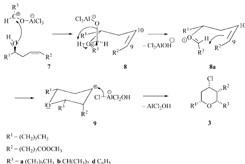
Scheme 1. Mechanism of the AlCl_3 -catalyzed Prins-type cyclization of methyl ricinoleate ( 1 ) and heptanal ( 2a ), isobutyraldehyde ( 2b ) and benzaldehyde ( 2d ).
