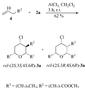
Figure 1. AlCl 3 -induced Prins-type cyclization of methyl 10-undecenoate ( 4 ) with heptanal ( 2a ) to give a diastereomeric mixture of rel -(2 S ,3 S ,4 S ,6 R )- 3a and rel -(2 S ,3 R ,4 S ,6 R )- 3a in a ratio of 2.6:1. In contrast to the reaction of methyl ricinoleate ( 1 ) with 2a a racemic mixture of each diastereomer was obtained which is indicated by the used nomenclature of relative stereochemistry.
