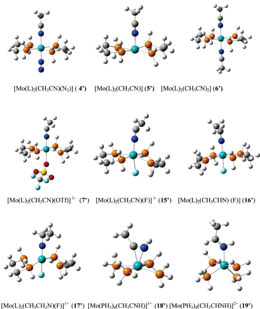
Figure 4. Optimized structures of the model systems ( \text{L} = \text{H}_2\text{P}-\text{CH}_2-\text{CH}_2-\text{PH}_2 ).
