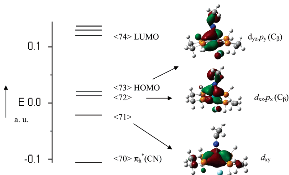
Figure 5. MO scheme of [\text{Mo}(\text{H}_2\text{P}-\text{CH}_2-\text{CH}_2-\text{PH}_2)_2(\text{CH}_3\text{CN})(\text{F})]^{-} ( 15' ).
