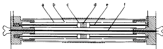
FIG. 4. Heated conductivity rig showing two of the five sample positions around the central tightening rod. (a) Glass tube; (b) water vapor escape hole; (c) Pt-black Ag electrode; (d) sample; (e) steel rod; (f) tightening rod.
