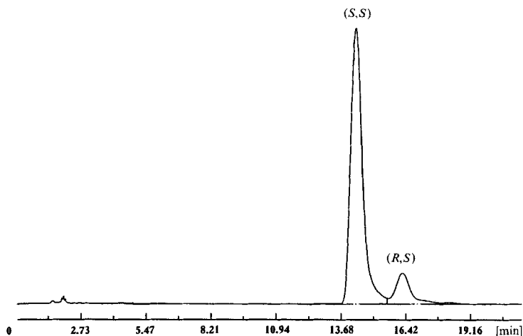
Fig. 1. HPLC Analysis of the protected dipeptide derivative 15 . Conditions: 10 \mu g applied; Lichrosorb SI60 (5 \mu m, 4.6 \times 150 mm); EtOH/heptane (1:9), flow rate 1 ml/min; detector 205 nm. (S,S)-Diastereoisomer: t_R 14.29 min, rel. area 87.4%. (R,S)-Diastereoisomer: t_R 16.26 min, rel. area 12.6%.
