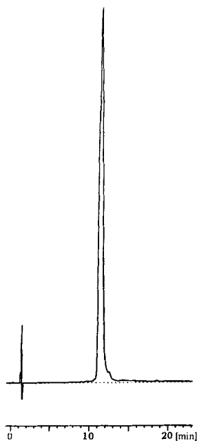
Fig. 2. HPLC Analysis of peptide 16 . Conditions: Milipore Delta Pak (5 \mu m, C_{18} 300 \text{\AA} , 3.9 \times 150 mm); 20 \rightarrow 40% MeCN/H _2 O (0.01% \text{CF}_3\text{COOH} ) gradient within 30 min, flow rate 1 ml/min; detection 210 nm.
