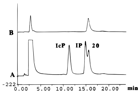
Figure 7. (A) Formation of glucose inositol phosphate as observed by HPAEC-PAD on Carboxack PA1. Identities of peaks are t_R 2.8 min, glucose, t_R 11.2 min, IcP; t_R 15 min, IP; t_R 15.5 min, compound 20. (B) HPAEC of the purified 20. Chromatographic conditions are the same as in Figure 3.
