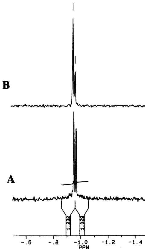
Figure 6. ^{31}\text{P} NMR spectra of Gro-PI ( 4 ) (A and B). Spectrum A shows the product obtained by transesterification of glycerol with IcP. Spectrum B was acquired after adding the diastereomerically pure Gro-PI, obtained by deacylation of PI, to the sample shown in trace A.
