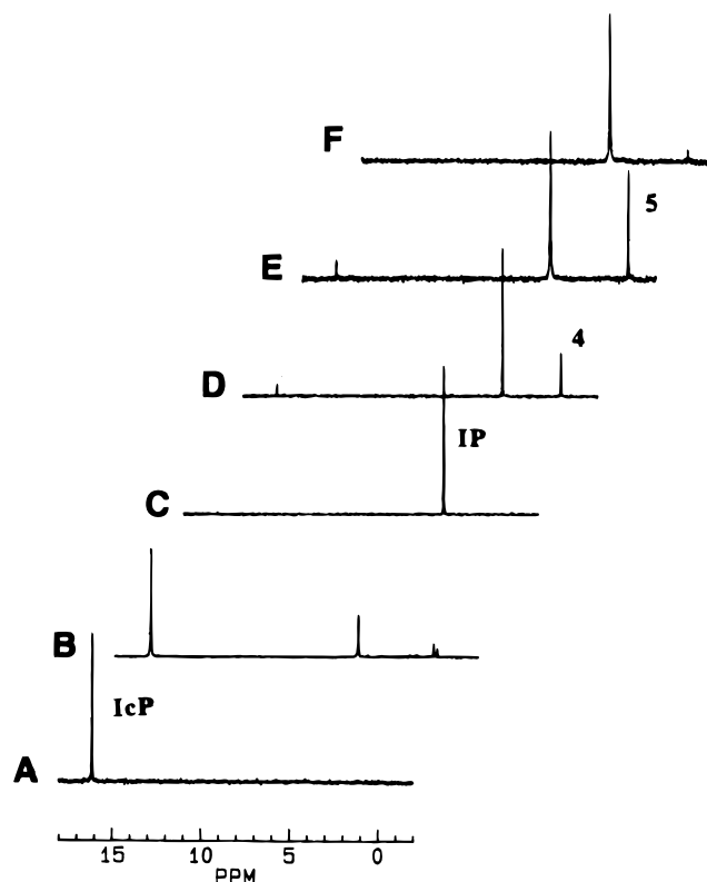
Figure 1. 31 P NMR spectra of reaction mixtures of IcP and PI-PLC under the following conditions: (A) IcP (10 mM) in Tris-HCl (70 mM) and EDTA (10 mM) buffer; (B) sample of DPPI (10 mM) dispersed with sodium deoxycholate (0.1 M) in Tris-HCl (0.2 M) 17 h after addition of PI-PLC from B. cereus (3.5 μg); (C) sample of IcP (10 mM) in 70 mM MOPS-Na, 10 mM EDTA treated with dialyzed PI-PLC; (D) same as trace C, but in the presence of 0.5 M glycerol; (E) same as the trace C, but in the presence of 0.5 M Tris-HCl; and (F) same as C, but after 16 days. All experiments were performed at pH 7.0.
