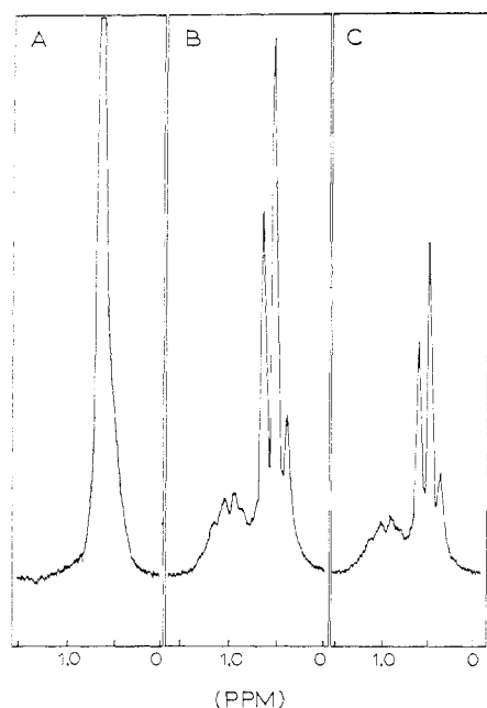
Figure 4.—Proton magnetic resonance spectra of propyldifluoroboranes. Chemical shift scale is relative to external tetramethylsilane: (A) product from tetraisopropyltin and boron trifluoride; (B) product from tetra- n -propyltin and boron trifluoride; (C) product of addition of difluoroborane to propene.
