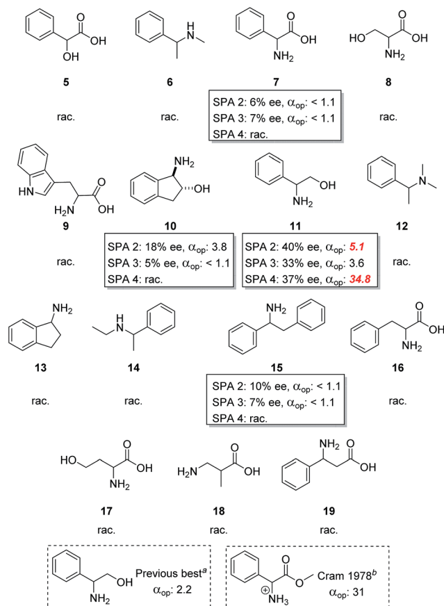
Fig. 3 Screening of compound classes. Conditions: all extraction experiments were conducted in 2 ml auto-sampler vials with crimp cap seals equipped with stirrars. A solution of the racemic guest (0.4 ml, 2 mM) dissolved in a phosphate buffer solution (buffer strength 0.1 M, pH 5.0) was carefully added to a solution of the corresponding host in chloroform (0.4 ml, 1.0 mM). The two-phasic system was then cooled to 6 °C and stirred at 900 rpm for 16 h. The phases were then allowed to separate over a period of 2 min. The aqueous phase was then removed and an aliquot injected into a reverse phase HPLC for determination of the ee, distribution and \alpha_{op} . All extraction experiments were carried out in triplo and with a simultaneous blank reaction (concentration of host = 0.0 mM). a See ref. 43. b See ref. 50.
