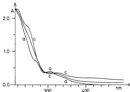
Fig. 2. Spectral changes during the photolysis of 2.07 \times 10^{-4} \text{ M} \text{Pd}^{\text{II}}(\text{1,5-COD})\text{Cl}_2 in EtOH at r.t. after 0 (a), 4 (b) and 16 (c) min irradiation time with white light (Osram HBO 100 W/2); 1 cm cell.
