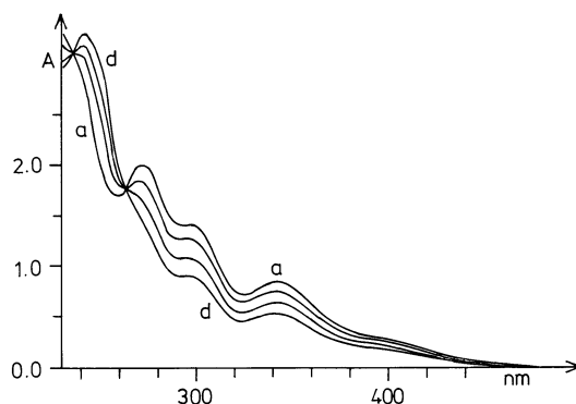
Fig. 3. Spectral changes during the photolysis of 4.36 \times 10^{-4} \text{ M} \text{Pd}^{\text{II}}(\text{1,5-COD})\text{Cl}_2 in \text{CH}_3\text{CN} at r.t. after 0 (a), 20 (b), 40 (c) and 100 (d) min irradiation time with white light; 1 cm cell.
