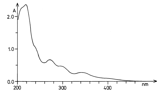
Fig. 1. Electronic absorption spectrum of 1.46 \times 10^{-4} \text{ M} \text{Pd}^{\text{II}}(\text{1,5-COD})\text{Cl}_2 at r.t. in acetonitrile; 1 cm cell.
