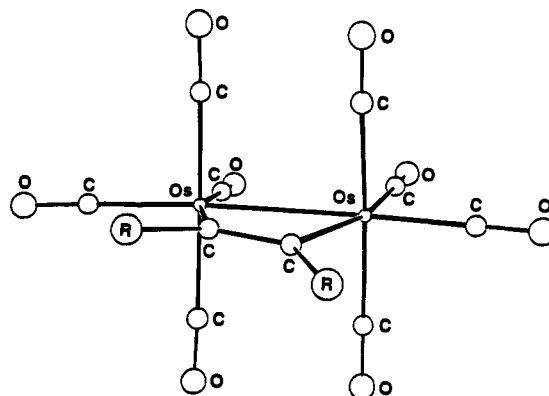
Figure 1. Schematic diagram of the molecular structure of \text{Os}_2(\text{CO})_8(\mu\text{-}\eta^1\text{-}\eta^1\text{-DMAD}) ; \text{R} = \text{CO}_2\text{Me} .
