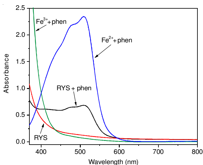
Fig. 3 Electronic absorption spectra of yellow reaction solutions (YRS) with and without addition of 1,10-phenanthroline; showing the existing of \text{Fe(II)} in yellow reaction solution
