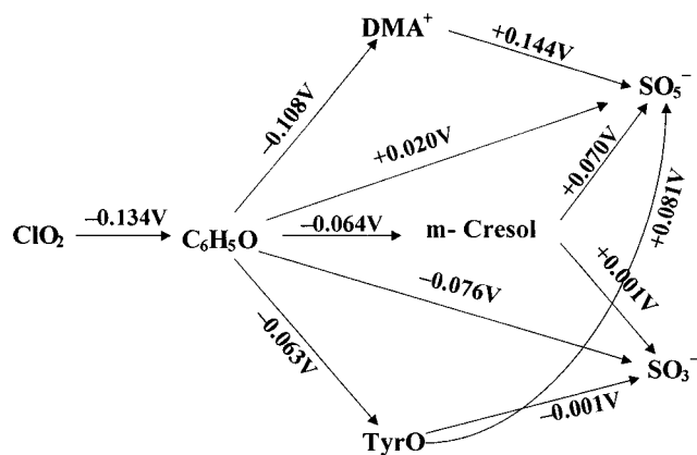
Figure 4. Redox relationships among the various species considered in this work in the derivation of the reduction potentials for \text{SO}_3^{\bullet-} and \text{SO}_5^{\bullet-} . The numbers represent the reduction potential differences, going left to right, between the redox pairs.
