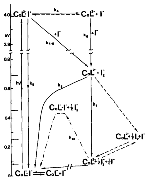
Fig. 3. Schematic representation of the energetics of the reactions that follows the \text{Co(EDTA)}^- - \text{I}^- system. L is EDTA.
