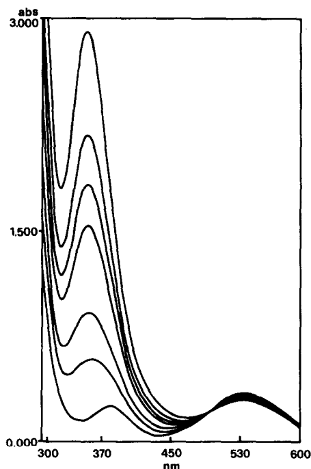
Fig. 2. Change in the absorption spectrum of an aqueous solution containing Co(EDTA) - ( 1.35 \times 10^{-3}\text{ M} ) and I - (0.5 M) with irradiation time.
