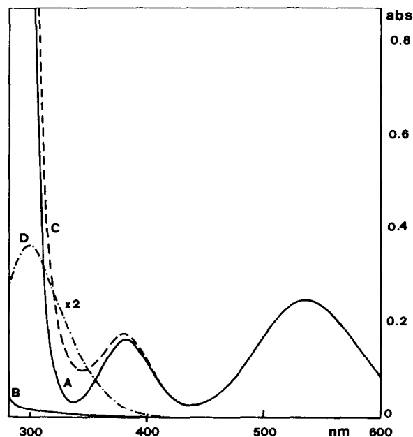
Fig. 1. Spectra of aqueous solutions of \text{K[Co(EDTA)]} in absence and in presence of KI. (A), [\text{Co(EDTA)}^-] = 1 \times 10^{-3} ; (B) [\text{I}^-] = 0.5 ; (C) [\text{Co(EDTA)}^-] = 1 \times 10^{-3} and [\text{I}^-] = 0.5 ; (D) absorbance difference between spectra C minus A. Optical path = 1 cm.
