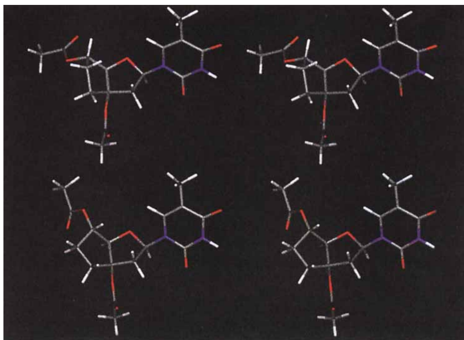
Fig. 4. Stereoscopic views of energy-minimized conformers of 5'-epi-bicyclocthyminidine 7 : conformers 7A (top) and 7B (bottom)
