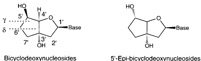
Fig. 1. Numbering scheme and composition of bicyclo- and 5'-epi-bicyclodeoxynucleosides
