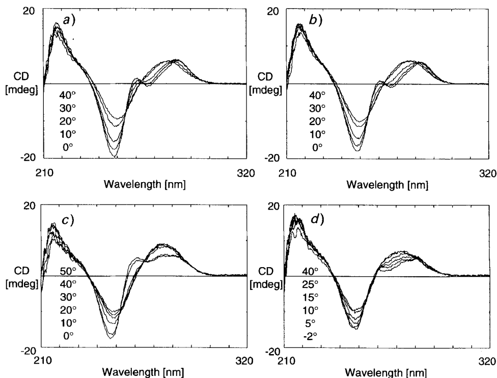
Fig. 6. CD Spectra of a) 15 · d ( A 10 ), b) 17 · d ( A 10 ), c) 21 ·bcd( T 10 ), d) 16 · 20 in 1M NaCl, 10 mM NaH 2 PO 2 (pH 7, c = 3.9–4.3 μmol)
