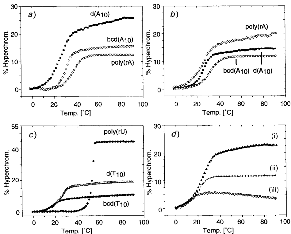
Fig. 5. UV/Melting curves of 1:1 mixtures of a) 15 , b) 17 , and c) 20 , with the complements indicated and of d) 15/19 (i), 17/21 (ii), 16/20 (iii) in 1 M NaCl, 10 mM NaH 2 PO 4 (pH 7, c = 3.9\text{--}4.3\text{ }\mu\text{mol} )
