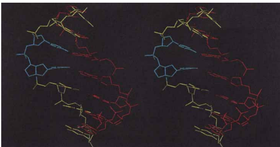
Fig. 7. Stereoscopic view of the average of the last 10 ps of a 200-ps dynamics trajectory of the duplex d(A-A-A-A-A-A) \cdot d(T-T-T-Y-T-T) ( Y = 5' -epi-bicyclodeoxythymidine). Solvent and H-atoms omitted, purine strand (red), pyrimidine strand (yellow), 5'-epi-bicyclodeoxythymidine modification (cyan).
