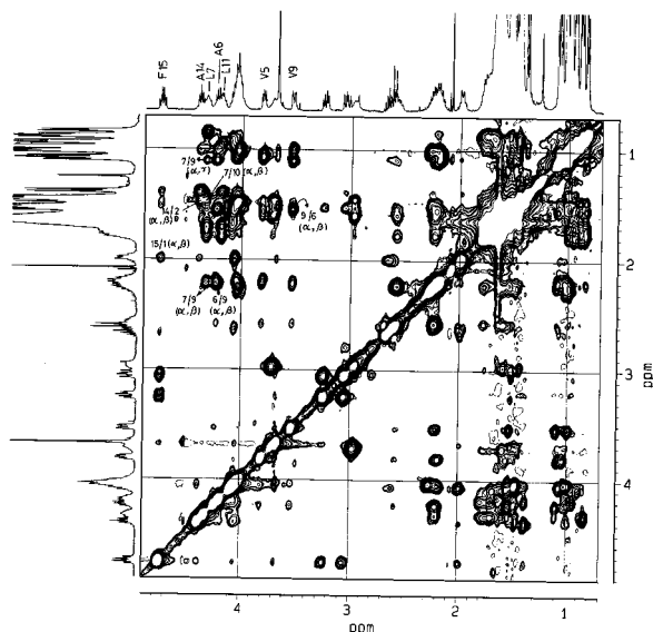
Fig. 7 Partial 400 MHz ^1\text{H} - ^1\text{H} NOESY spectrum of the peptide 1 in \text{CDCl}_3 . Some observed long range \text{C}'\text{H} \longleftrightarrow \text{C}'\text{H}/\text{C}'\text{H} \longleftrightarrow \text{C}'\text{H} NOE connectivities are indicated.
