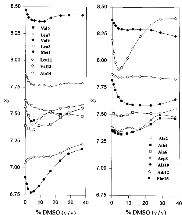
Fig. 4 Solvent dependence of chemical shifts of amide proton resonances of peptide 1 at varying concentrations of (\text{CD}_3)_2\text{SO} in \text{CDCl}_3
