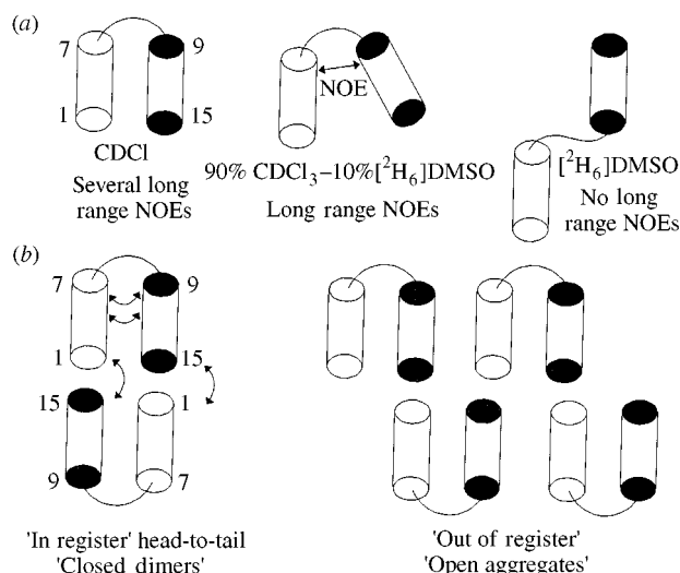
Fig. 8 Schematic representations of (a) solvent dependent structural changes of the peptide 1; (b) possible aggregation patterns for peptide 1 in CDCl 3
