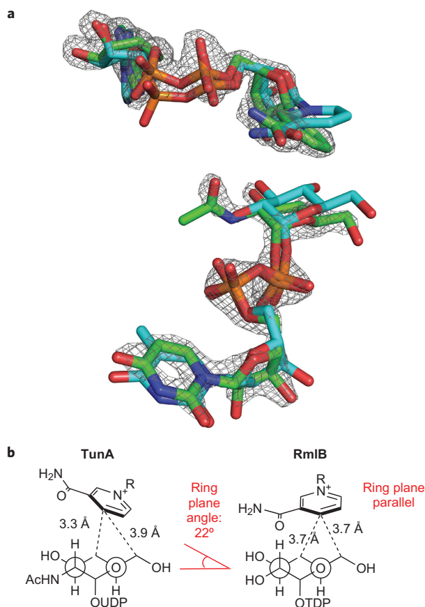
Figure 4 | Comparison of the conformations of substrates and cofactors in active sites between TunA and RmlB. a , Colour code for carbon atoms: green, TunA; blue, RmlB. Electron density maps are 2F_o - F_c syntheses (grey) contoured at \sim 1\sigma ; no density data are available for RmlB. b , Schematic showing relative positions and angles of substrates and cofactors in active sites of TunA and RmlB. When compared with existing 4,6-dehydratases DesIV/RmlB, the \text{NAD}^+ nicotinamide and GlcNAc ring planes are no longer parallel and lie \sim 20^\circ to each other, yet are still positioned to allow efficient hydride-abstraction at C-4'' of UDP-GlcNAc. This subtle rotation plays an important role later in the catalytic cycle, during hydride return to the 4-keto-5,6-ene intermediate. Studies using dTDP-glucose complexed with DesIV have shown that orientation of the plane of \alpha,\beta -unsaturated intermediate closely mirrors that of the ring plane of the original substrate 29 . If extended to TunA, the altered position and ring plane of nicotinamide in TunA result in poor alignment for hydride return to C-6'' of the intermediate; instead, 1,2-delivery at C-4'' is favoured, followed by re-protonation of O-4'' by Tyr143 (Supplementary Fig. S15). From the determined structure these steps appear able to occur without a need for significant conformational changes.
