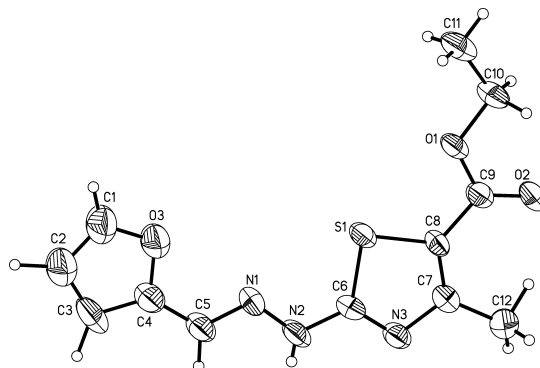
Fig. 2. ORTEP Drawing of Compound 8g
