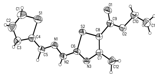
Fig. 3. ORTEP Drawing of Compound 8h
